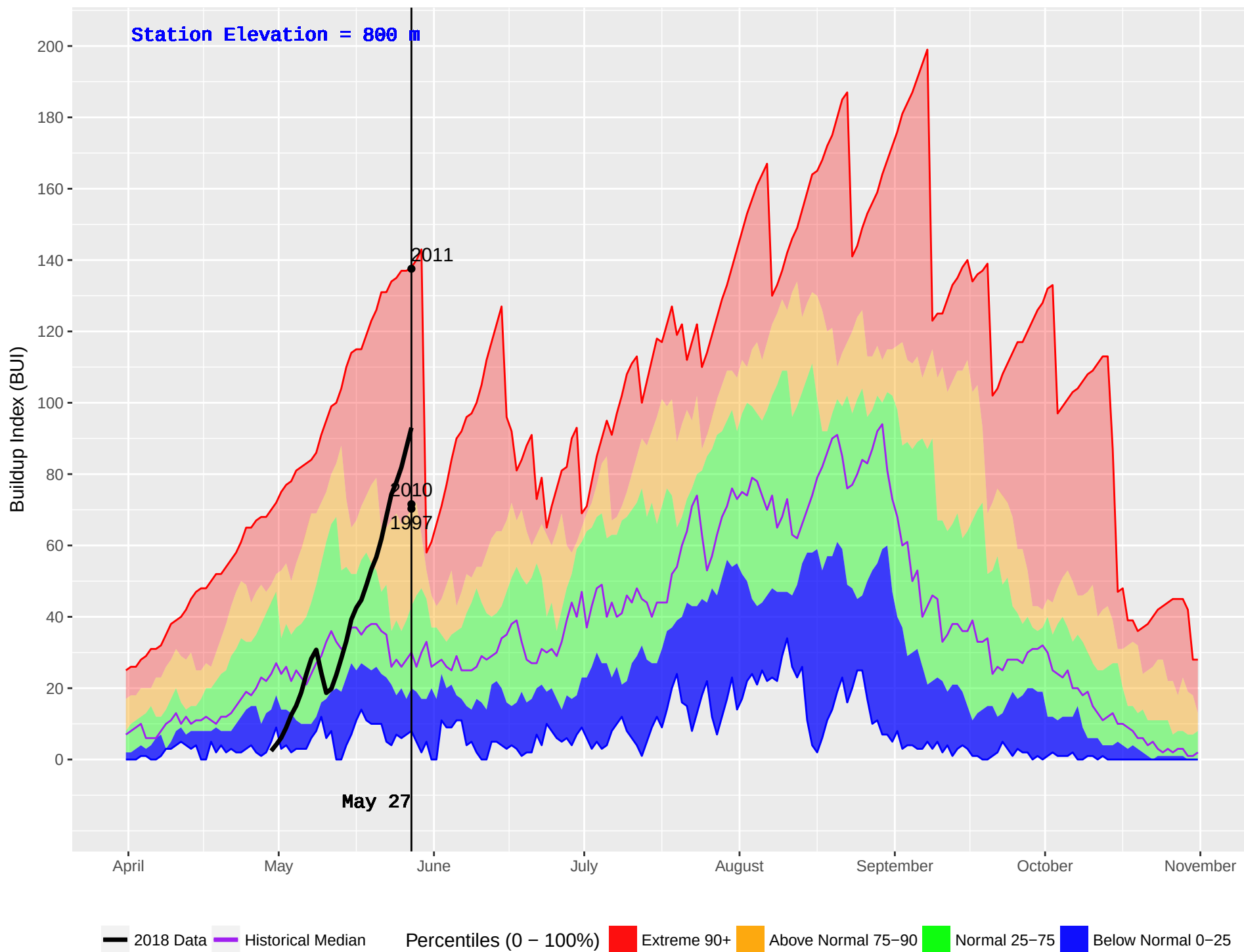
GOLD HILL (379) : Historical (1979–2016) and Current (2018) Noon Buildup Index (BUI)
